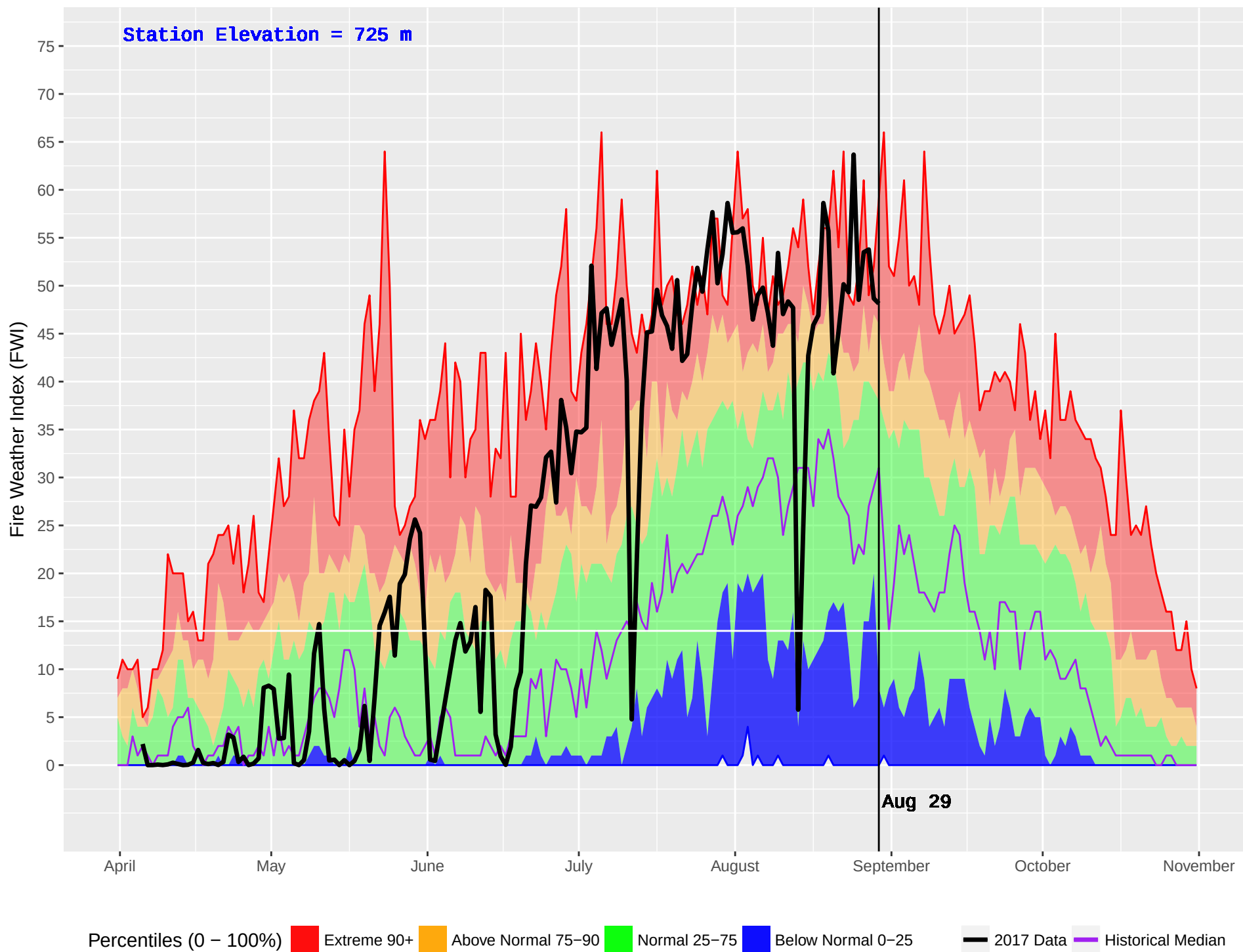
PENDOREILLE (402) : Historical (1986–2016) and Current (2017) Noon Fire Weather Index (FWI)
