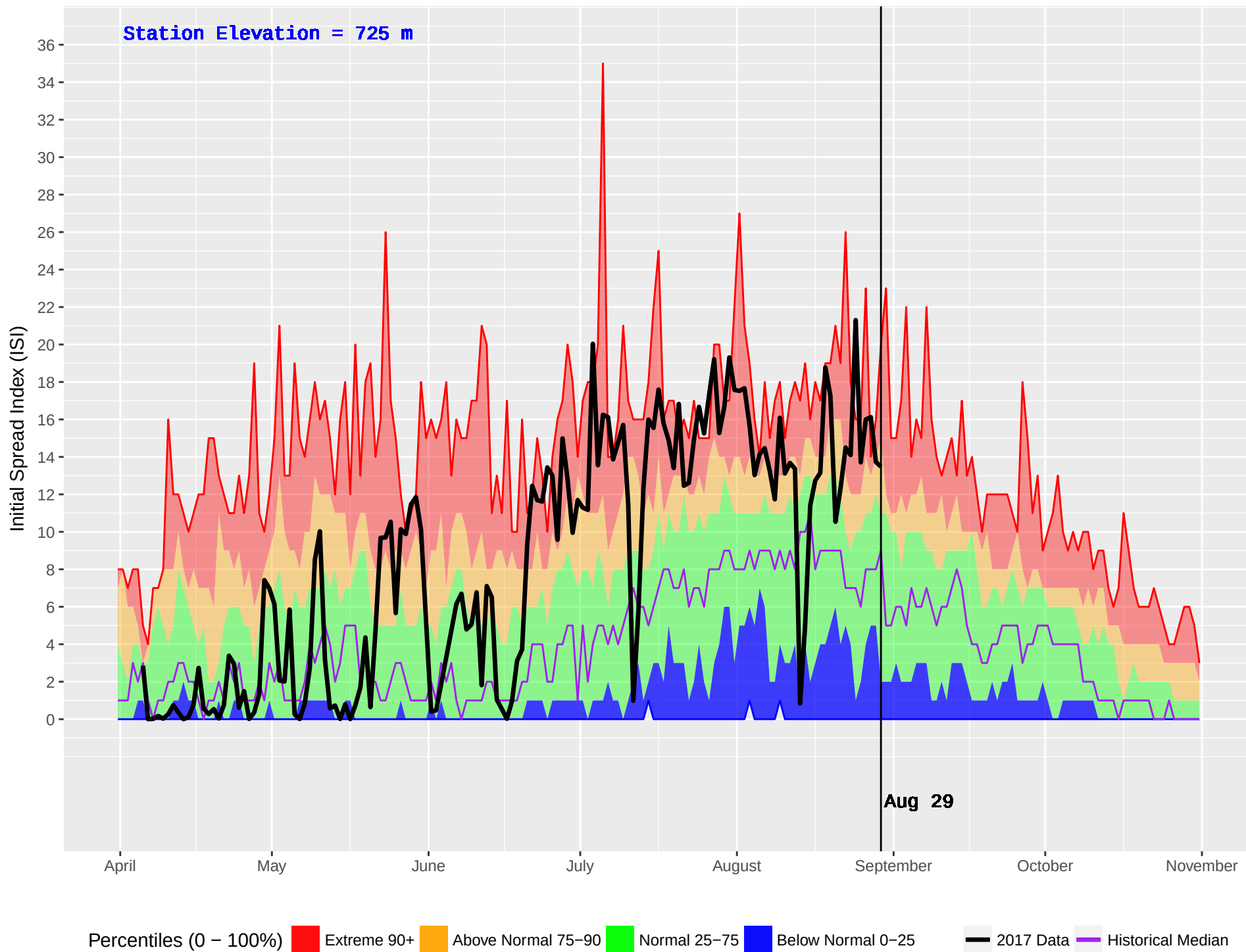
PENDOREILLE (402) : Historical (1986–2016) and Current (2017) Noon Initial Spread Index (ISI)
